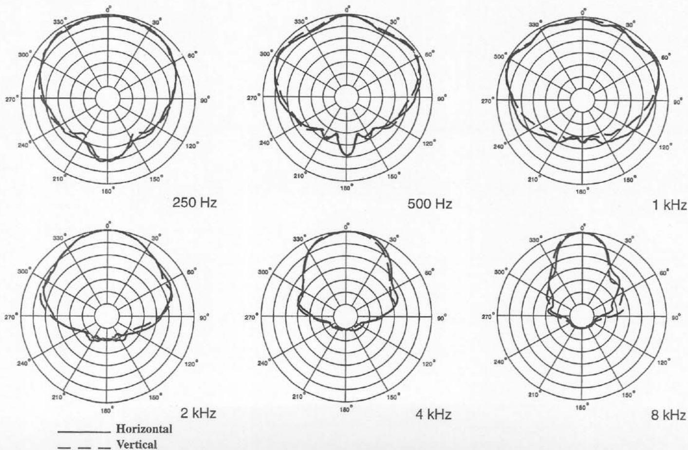
Figure 1—Polar Response
